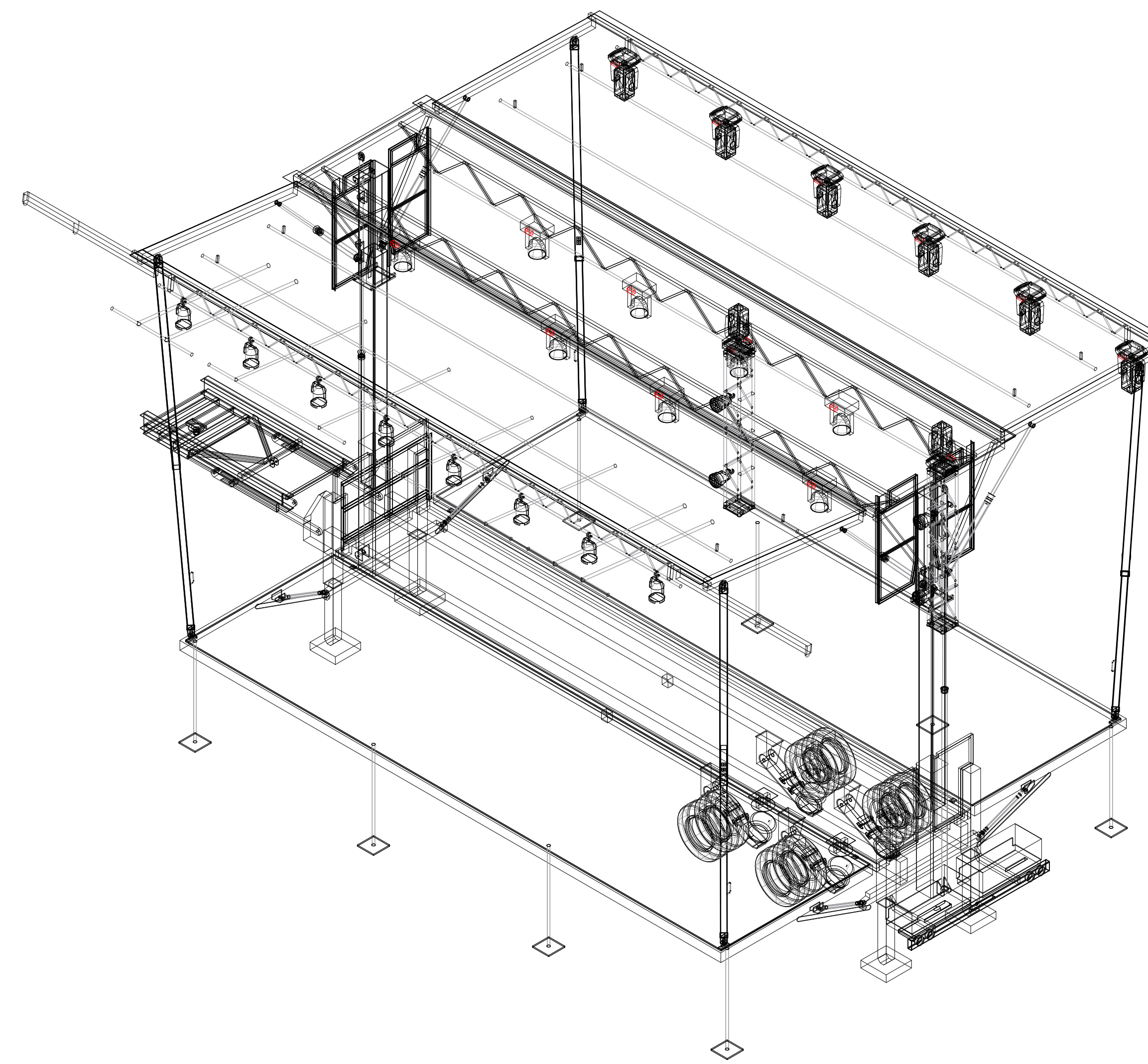
1-4 Lighting - Right Isometric Scale: 1/4" = 1'-0"
