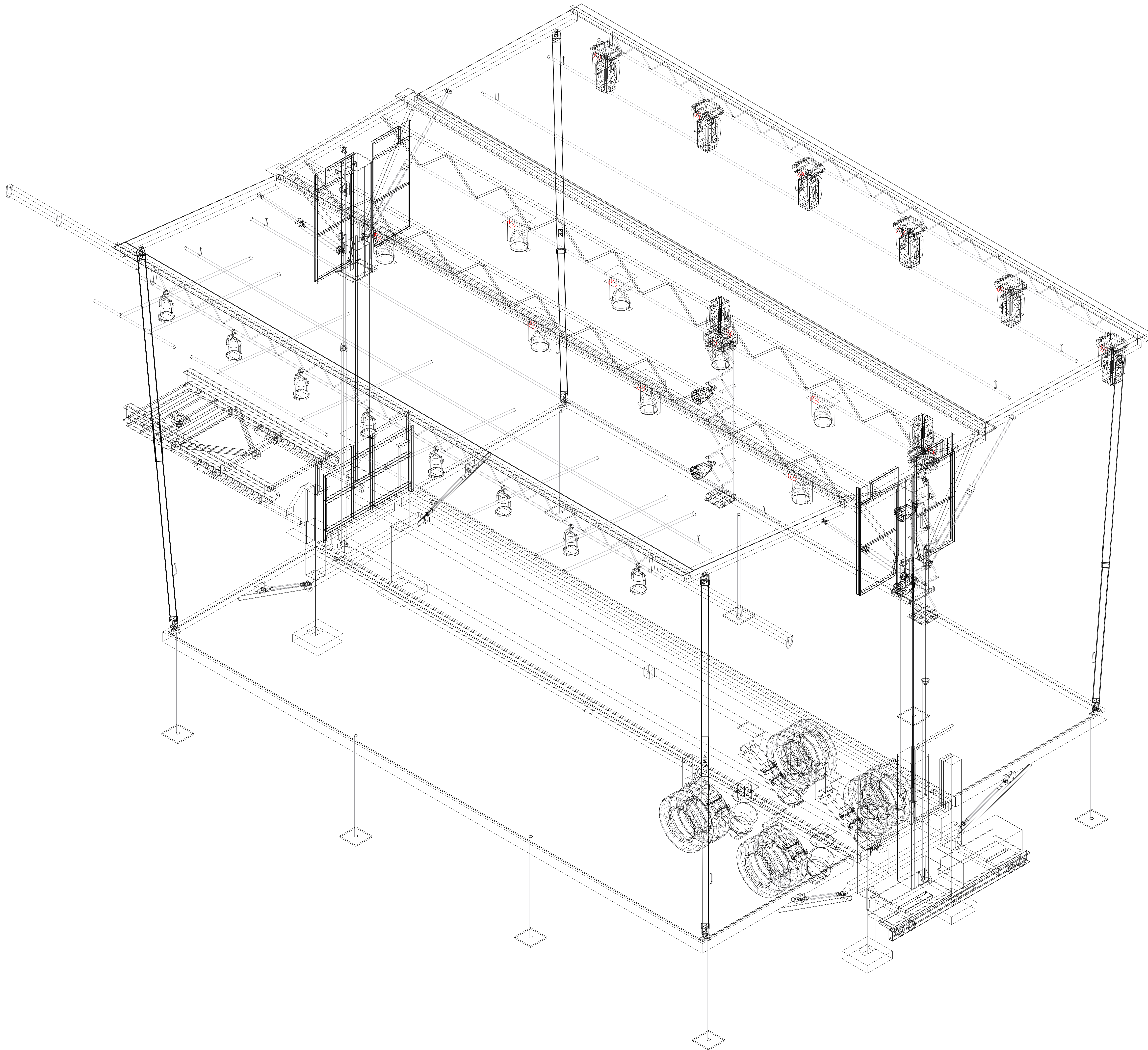
5-1 Lighting - Right Isometric Scale: 3/4" = 1'-0"
